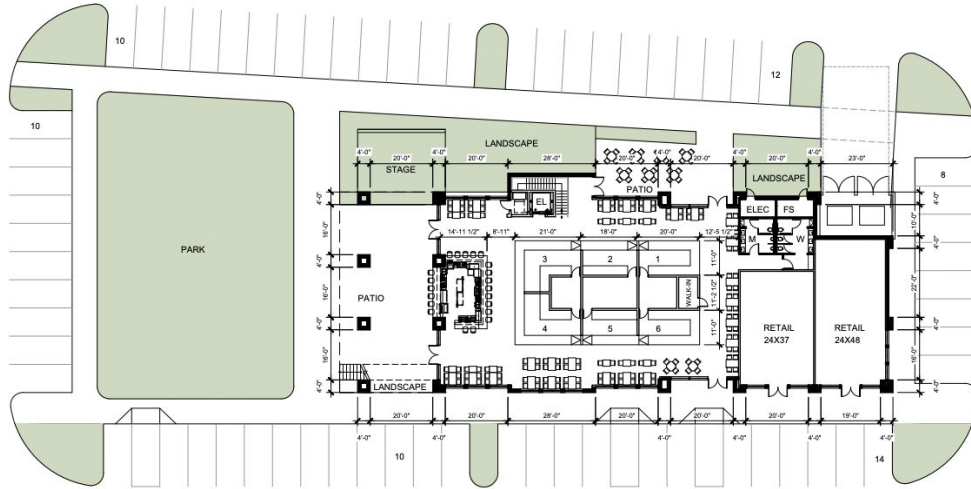
02 CONCEPTUAL 1ST FLOOR PLAN - BLDG 7 SCALE: 1/8"=1'-0"
